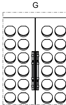
07.31.09 YAPRAK MENTEŞE LEAF HINGE
