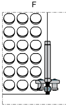
07.31.04 ALT KAFA ARABA BOTTOM END ROLLER
