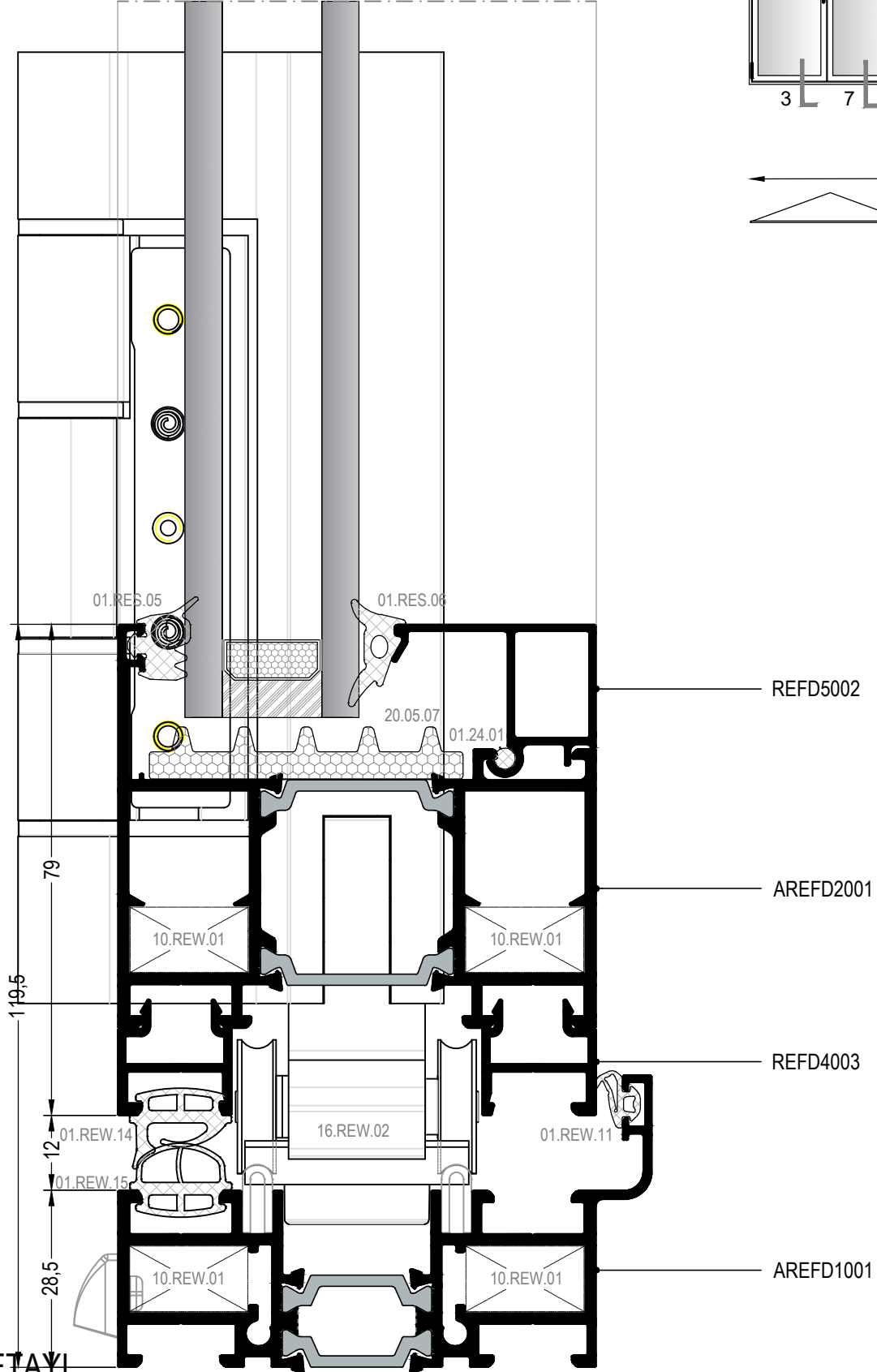
KATLANIR KAPI DIŐA AÇILIM DETAYI FOLDING DOOR OUTWARD OPENING DETAIL
