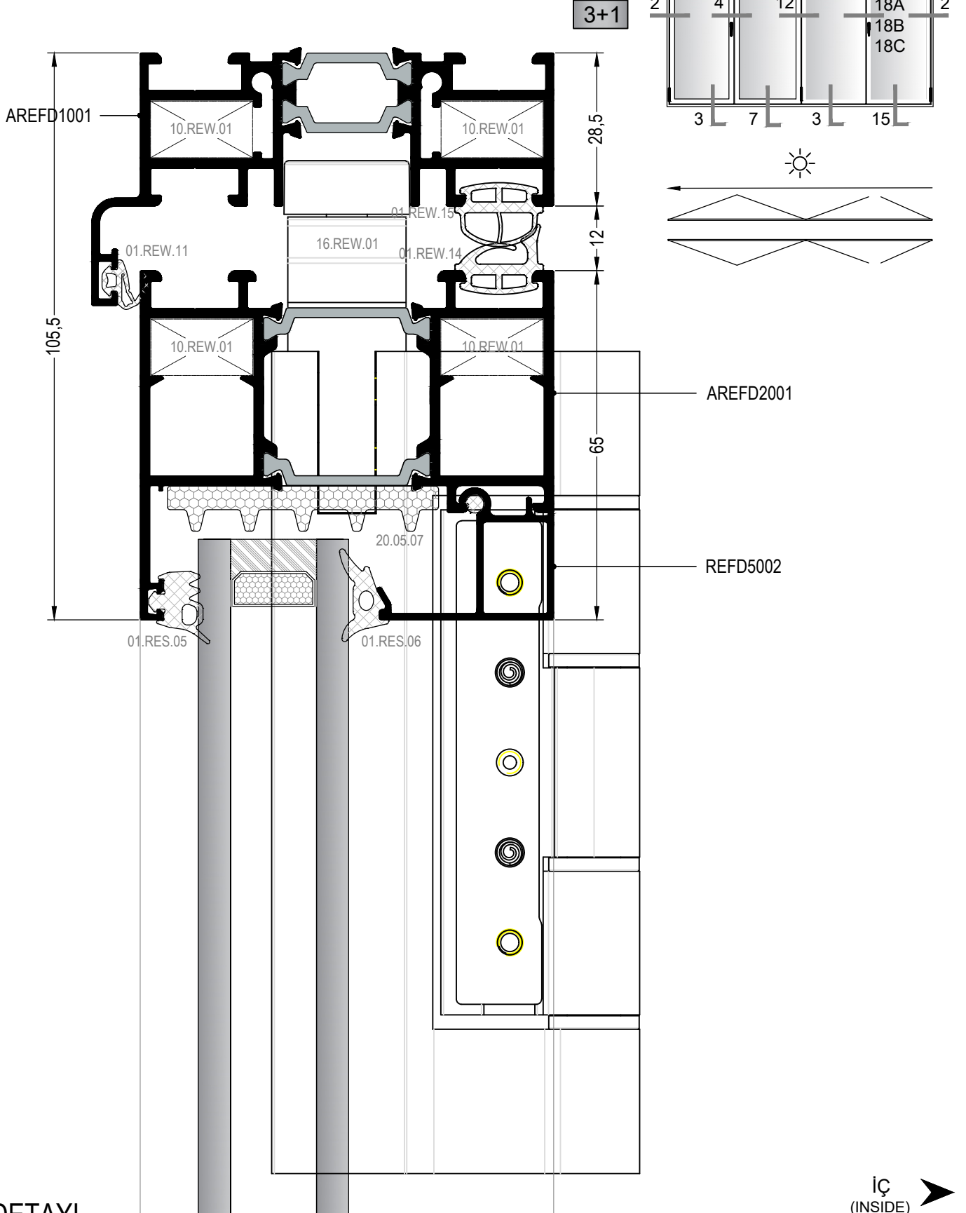
KATLANIR KAPI İÇE AÇILIM DETAYI FOLDING DOOR INWARD OPENING DETAIL
