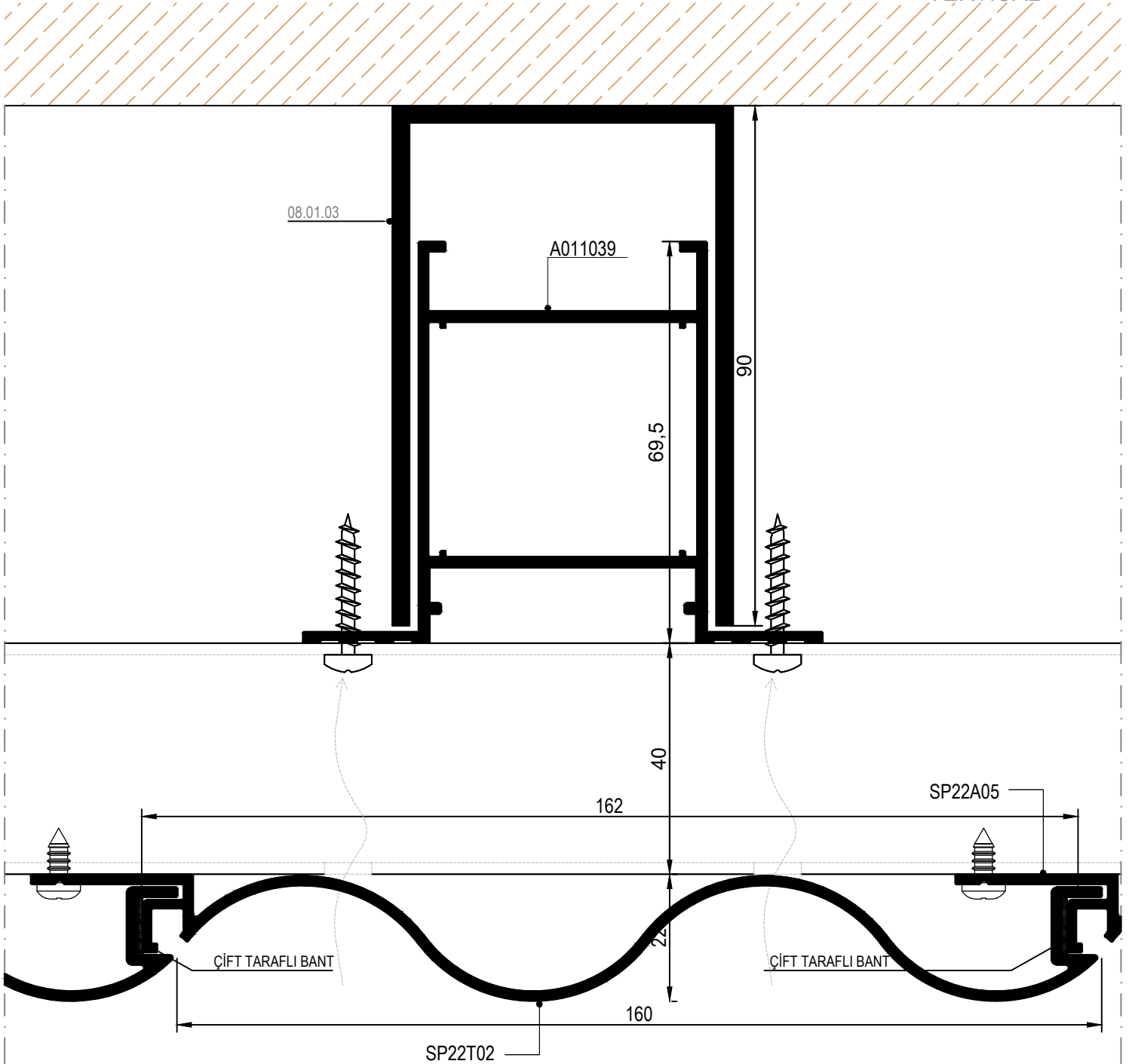
23 DETAYI DETAIL
