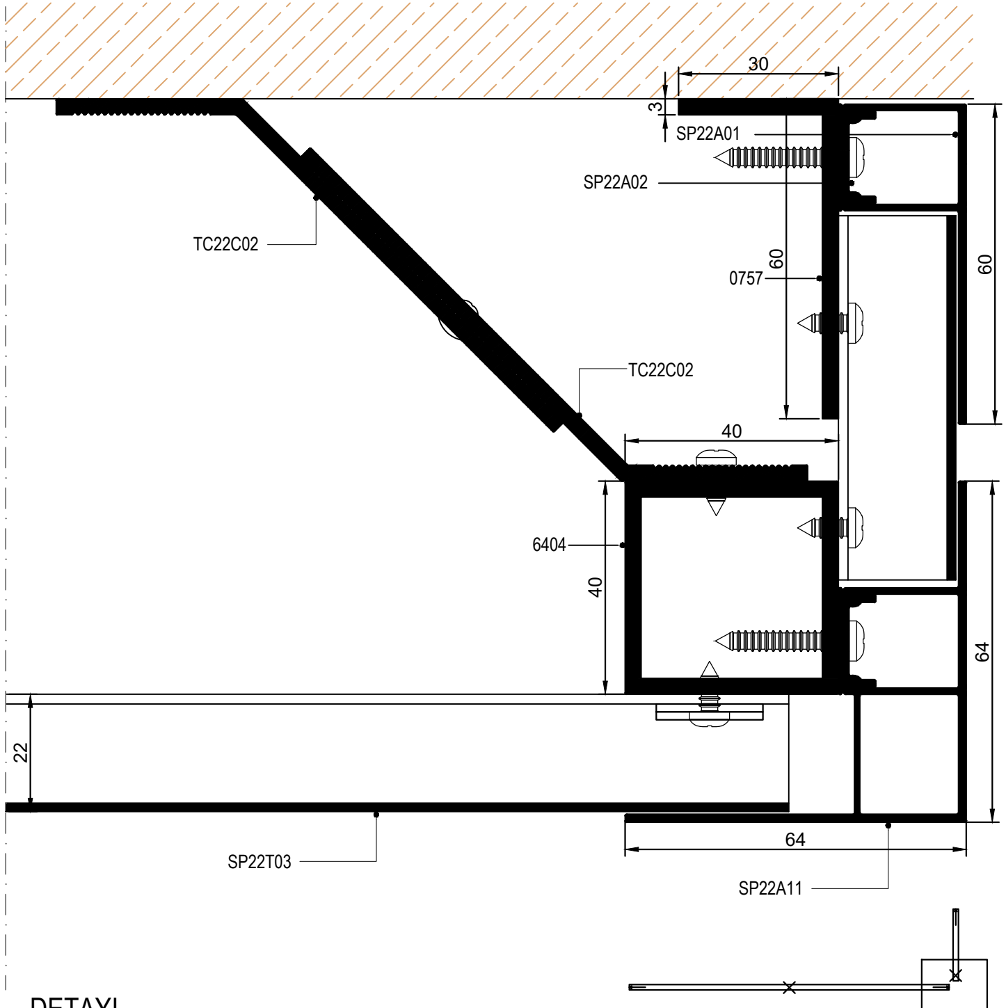
ISIL GENLEŞME SERBESTLİKLERİ THERMAL EXPANSION RELEASES
