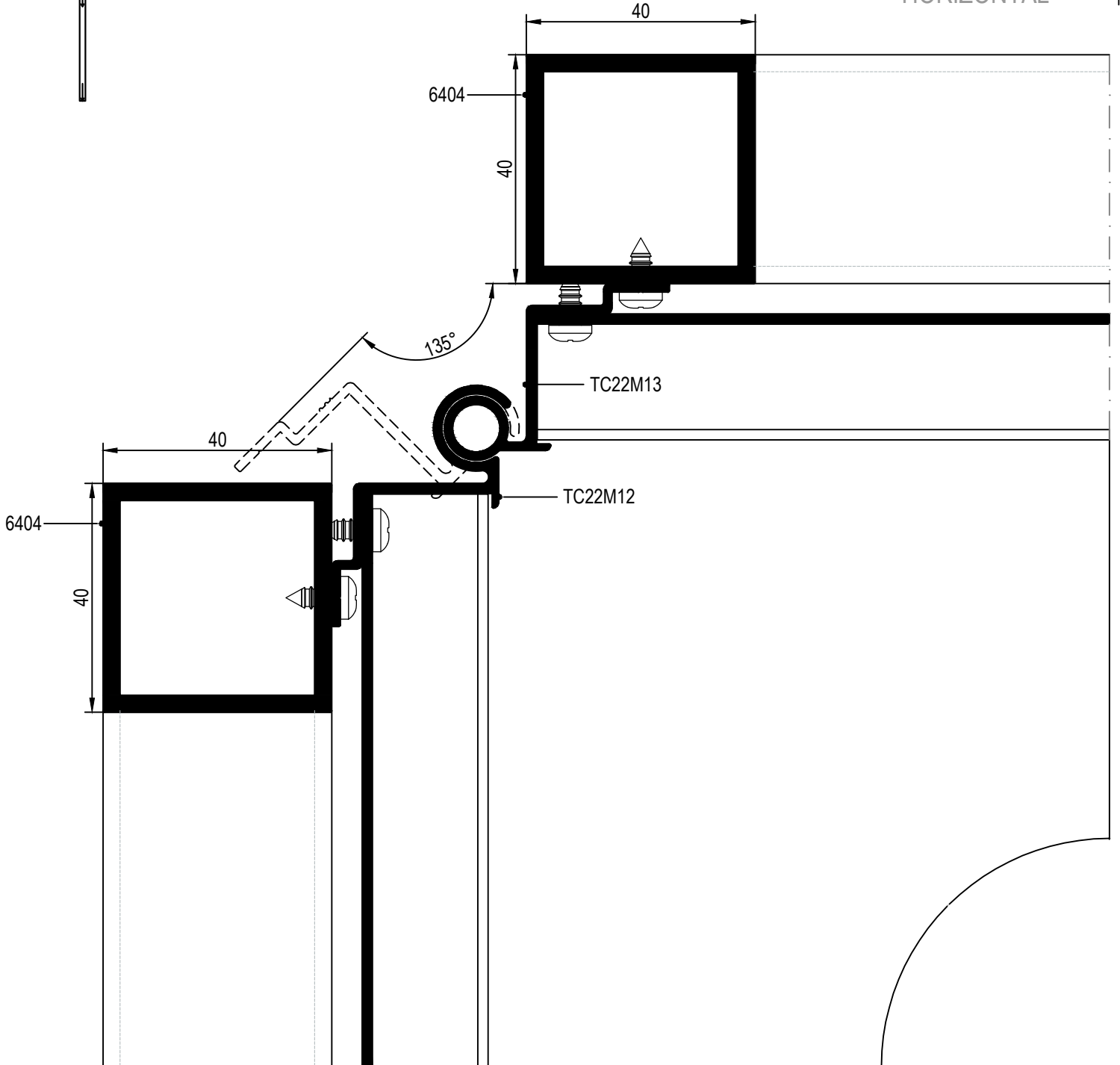
16 DETAYI DETAIL
