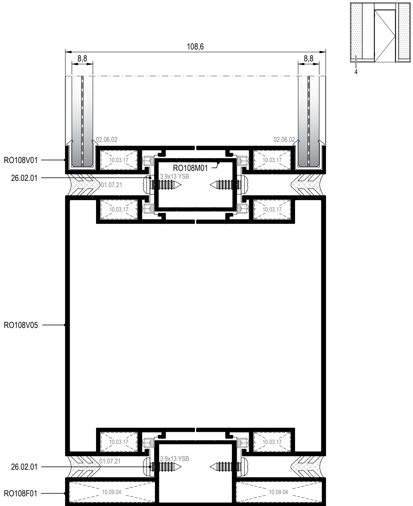
④ DETAYI DETAIL
