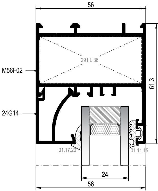
28 DETAYI DETAIL
