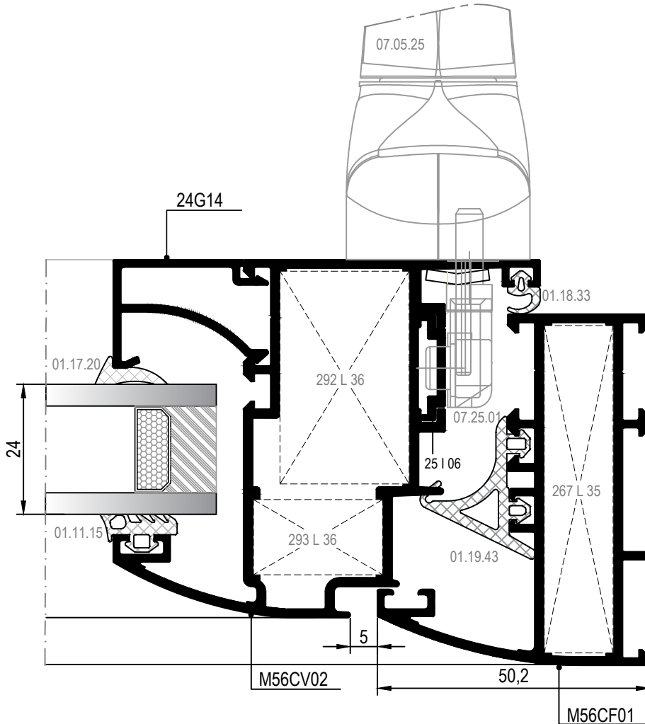
16 DETAYI DETAIL
