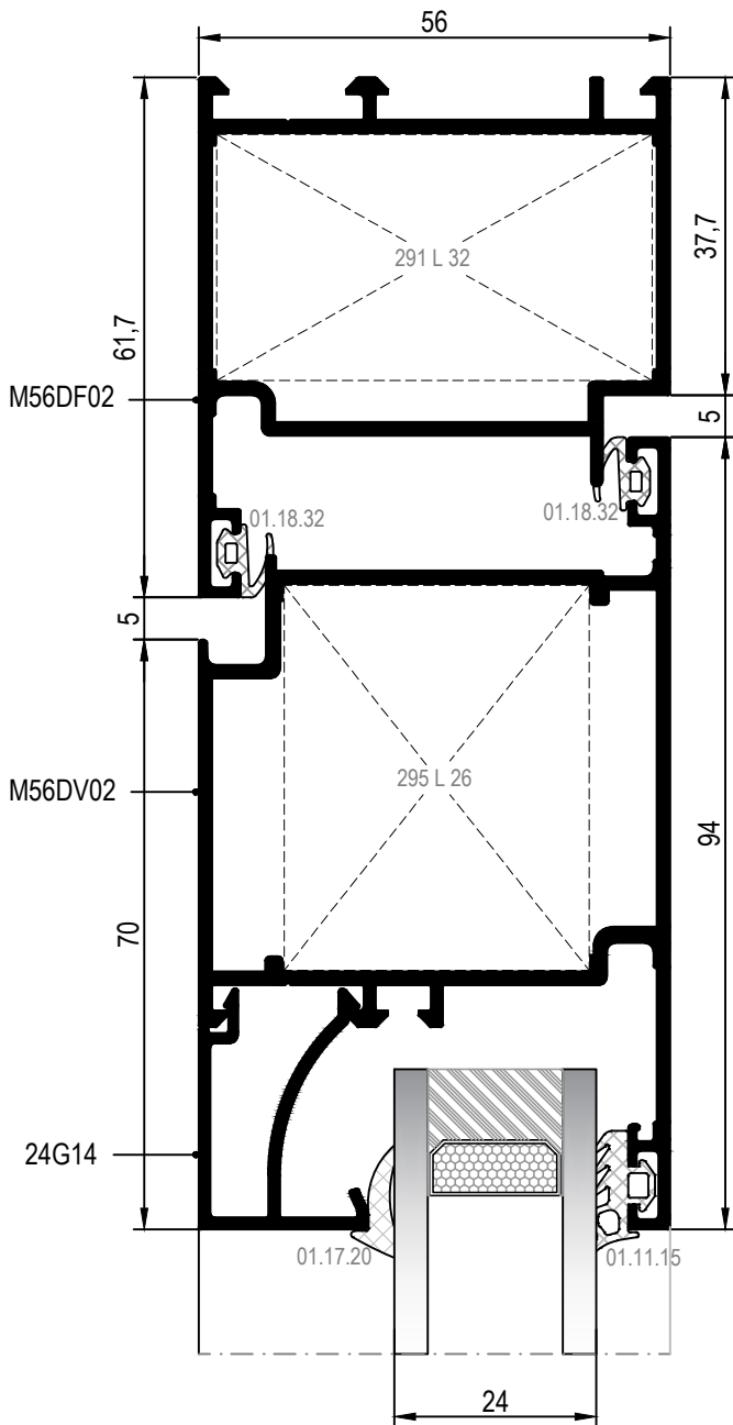
33 DETAYI DETAIL
