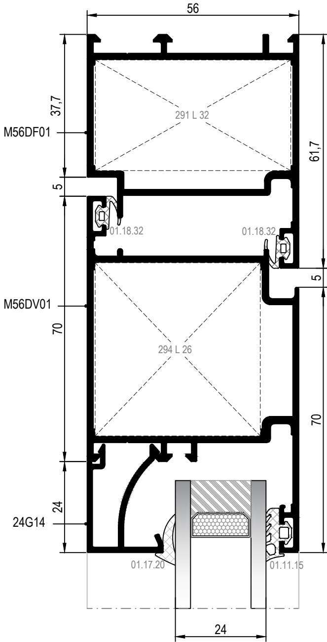
22 DETAYI DETAIL
