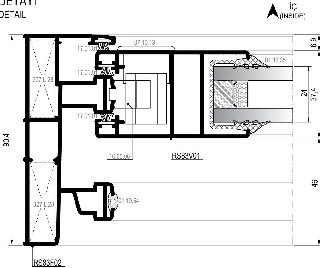
①A DETAYI DETAIL
