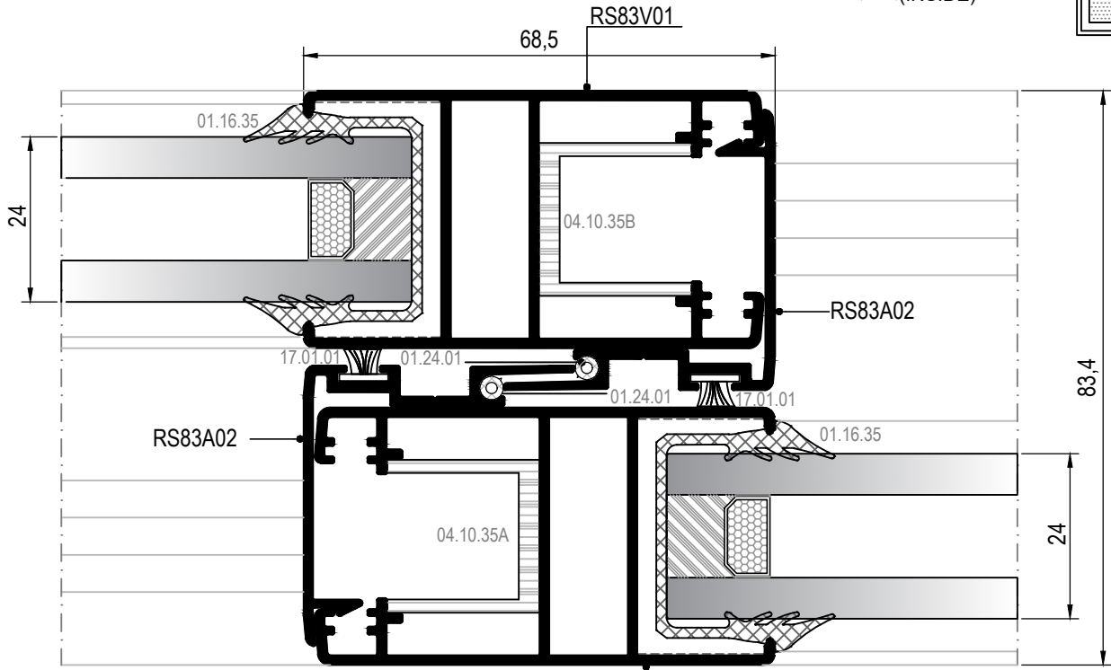
③ DETAYI DETAIL
