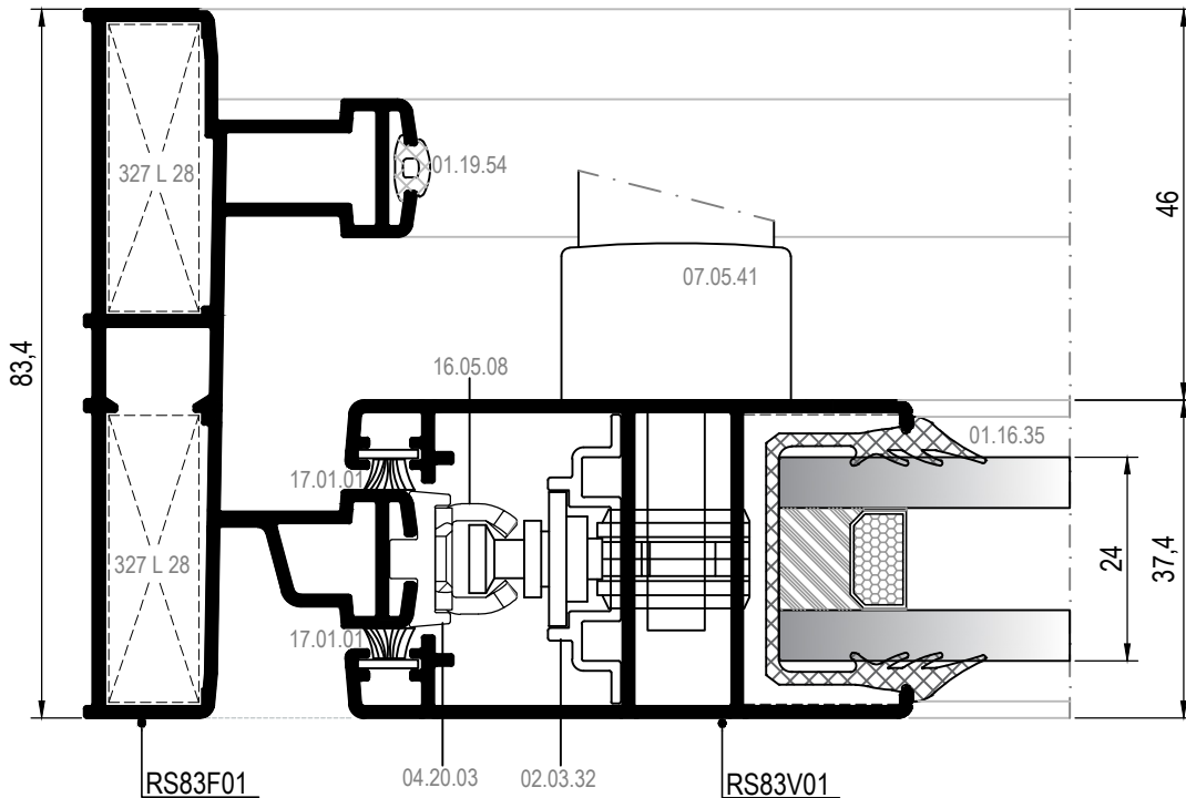
2B DETAYI DETAIL
