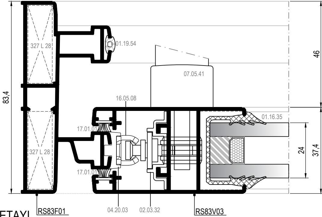
2A DETAYI DETAIL
