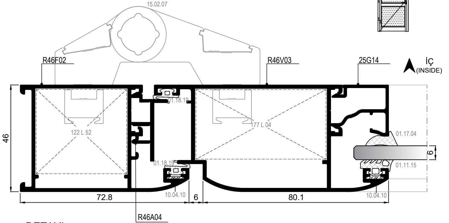
10 DETAYI DETAIL
