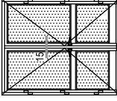
DIŐA AÇILIM HEMYÜZ KAPI DETAYLARI OUTWARD OPENING FLUSH DOOR DETAILS
