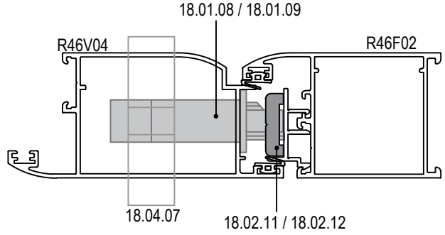
**DIŞA AÇILIM HEMYÜZ ADAPTÖRLÜ (R46 A 04) DETAY İÇİN **OUTWARD OPENING FLUSH DOOR DETAIL (R46 A 04)
