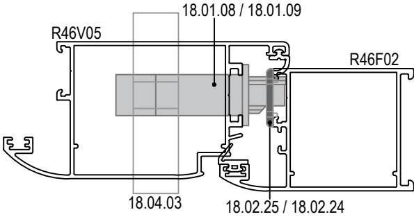
**İÇE AÇILIM BİNİLİ DETAY İÇİN **INWARD OPENING DOOR DETAIL
