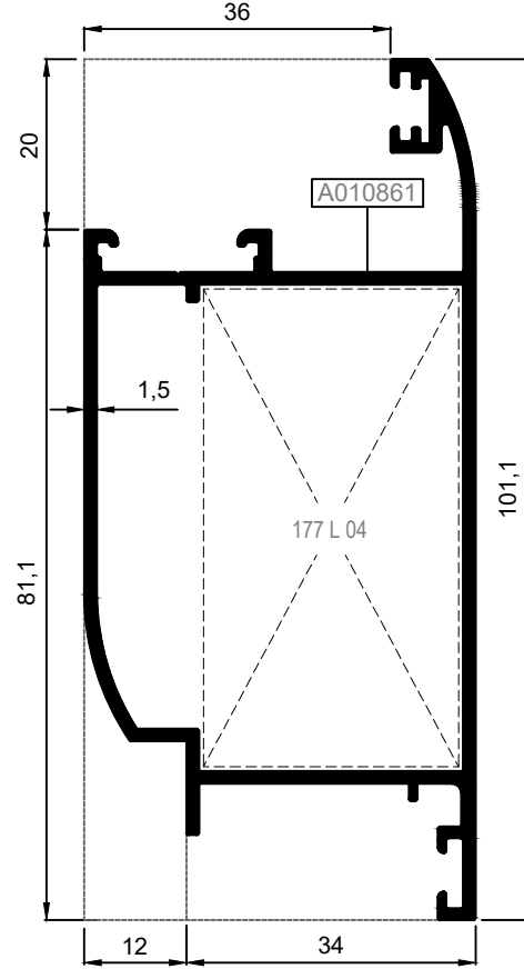
DIŞA AÇILIM HEMYÜZ KAPI KANAT PROFİLİ OUTWARD OPENING FLUSH DOOR VENT PROFILE
