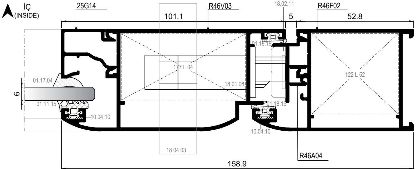
11 DETAYI DETAIL
