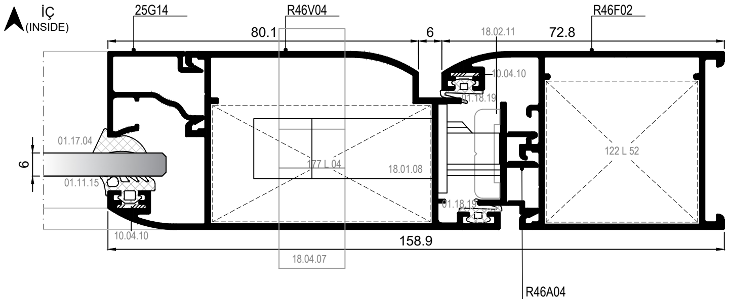
13 DETAYI DETAIL
