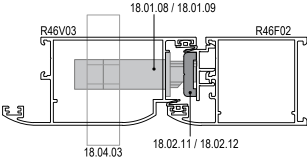
**İÇE AÇILIM HEMYÜZ ADAPTÖRLÜ (R46 A 04) DETAY İÇİN **INWARD OPENING FLUSH DOOR ADAPTER DETAIL (R46 A 04)
